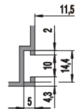
Frame groove 10/14
